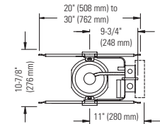
Top View (Electronic Ballast)
