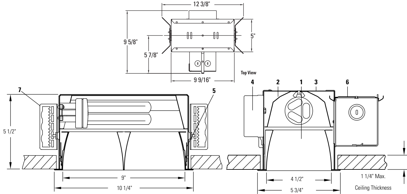
Ceiling Cutout: 5 1/8" L X 9 5/8" W
