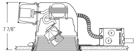
1161/1103R LyteSeal™ Non-IC Remodeler Ring
